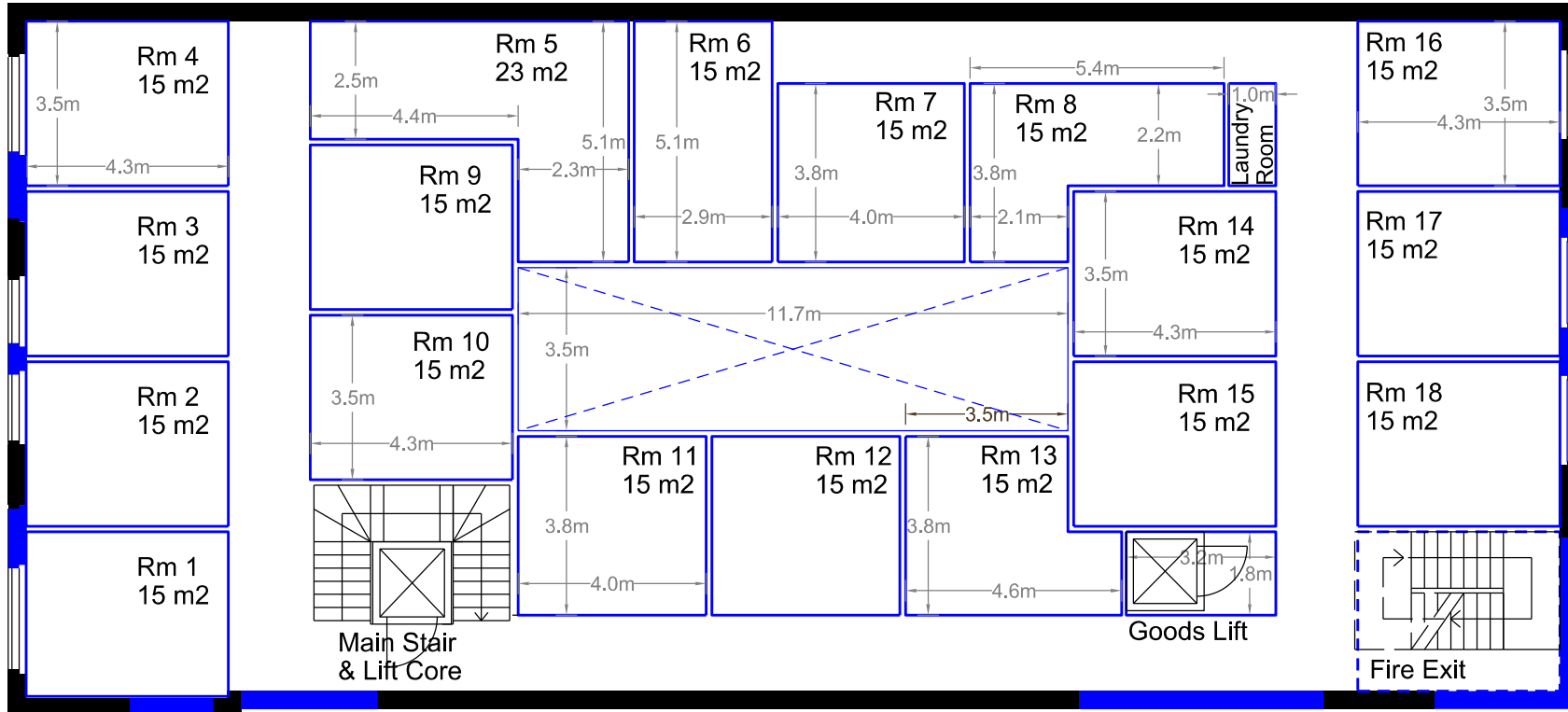
PROPOSED FIRST FLOOR (Option 1 rev F)
